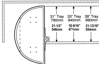
Minimum Inside Cabinet Depth
